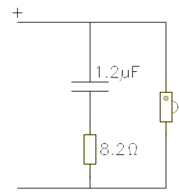
Impedance correction circuit
